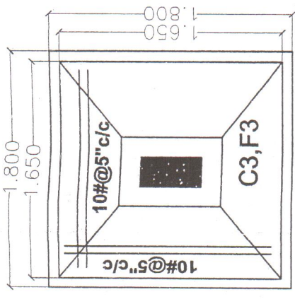
C3,F3 PLAN
